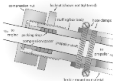
CUT-AWAY VIEW OF A STUFFING BOX ASSEMBLY
