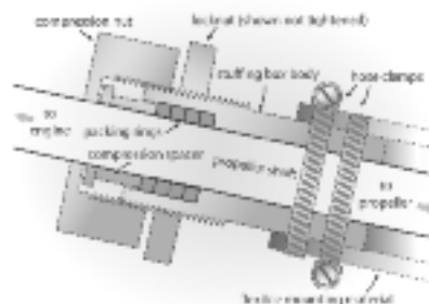
CUT-AWAY VIEW OF A STUFFING BOX ASSEMBLY
